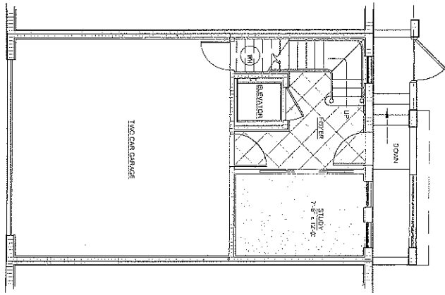
GROUND LEVEL TWO CAR GARAGE, STUDY & FOYER AC AREA: +/- 280 sq. ft. GARAGE AREA: +/- 430 sq. ft.
