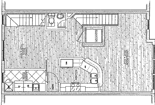
SECOND LEVEL LIVING ROOM, DINING ROOM, KITCHEN LAUNDRY ROOM, HALF BATH AC AREA: +/- 800 sq. ft.
